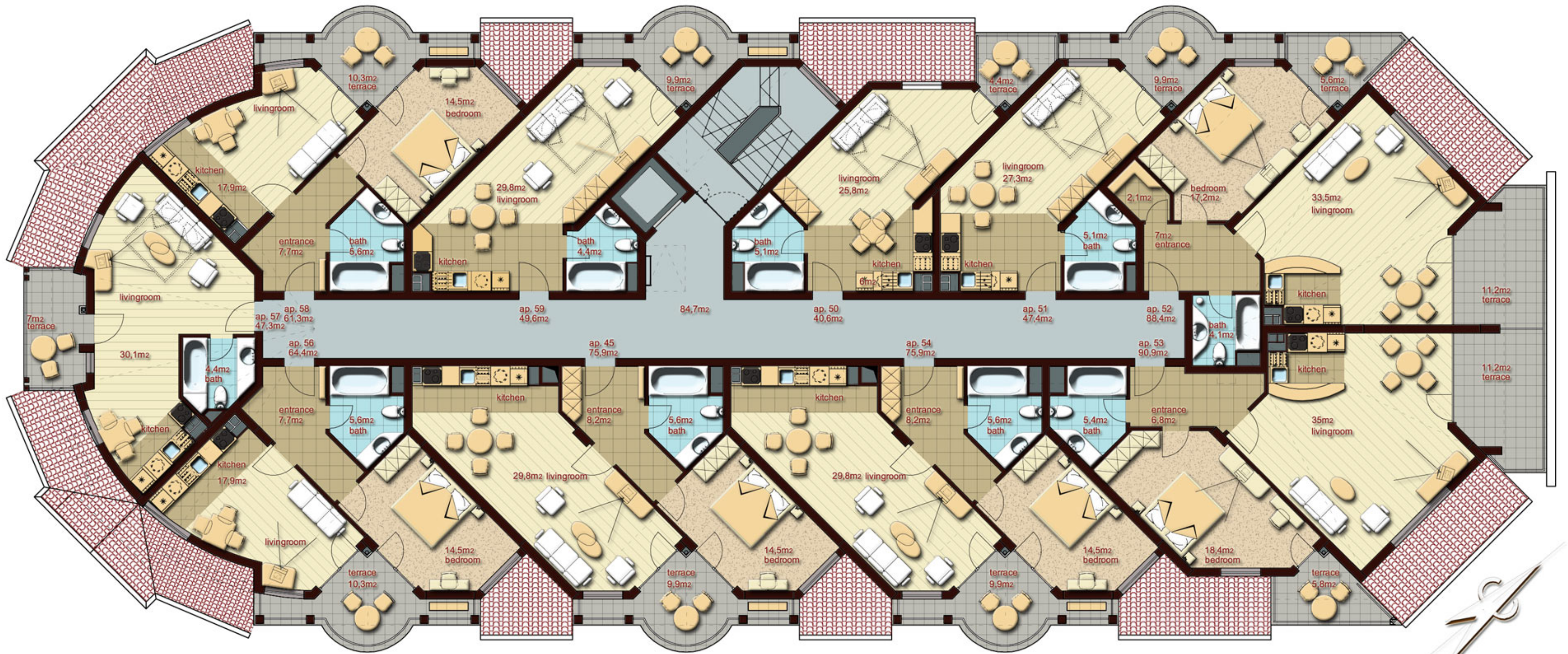
BLOCK 1; 6TH FLOOR
